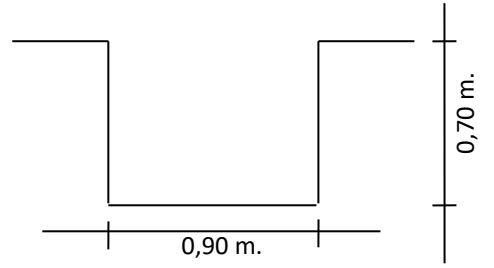
CANAL GENERAL RODEO
